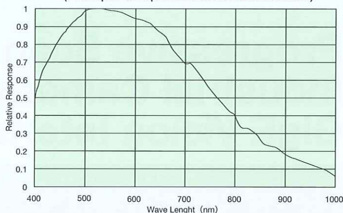
Spectrum sensitivity characteristic (Example of representative characteristic)
