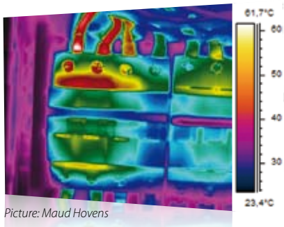
With the naked eye this circuit breaker looks fine, but in infrared it is clear that it is a highly dangerous situation. This circuit breaker needs to be replaced urgently.
